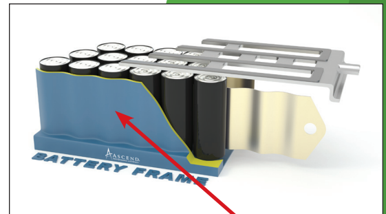
Battery frame supporting Li-ion cells
