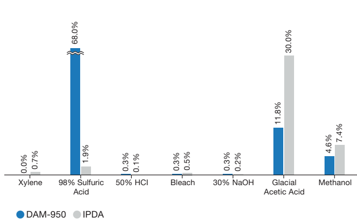
Chemical Resistance*
