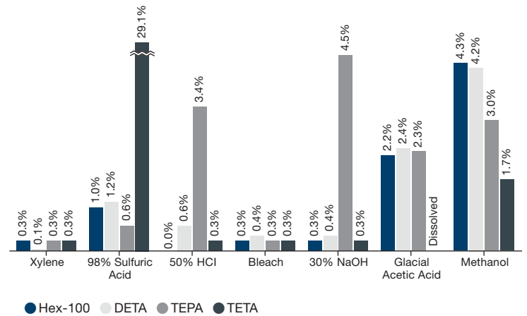
Chemical Resistance*
